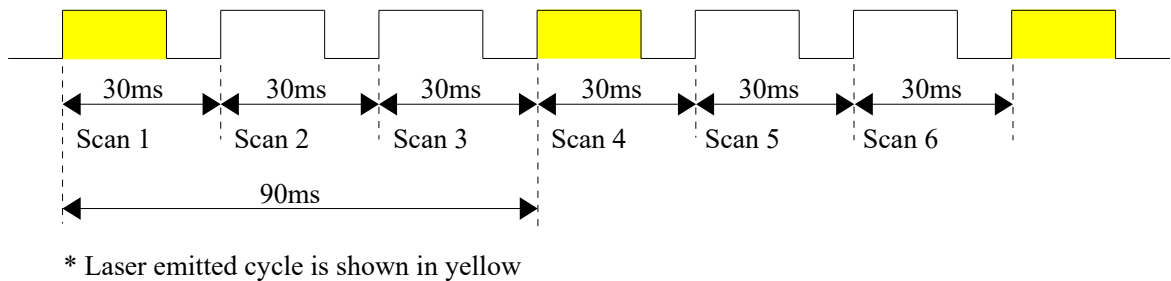
Figure 4-22 Operation of UAM when scan skip count is 2
