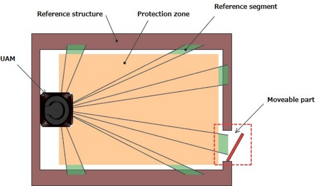
Figure 4-13 Top view of the area protection using reference monitor function
