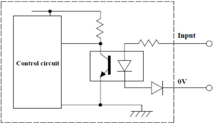
Figure 6-3 Input circuit
