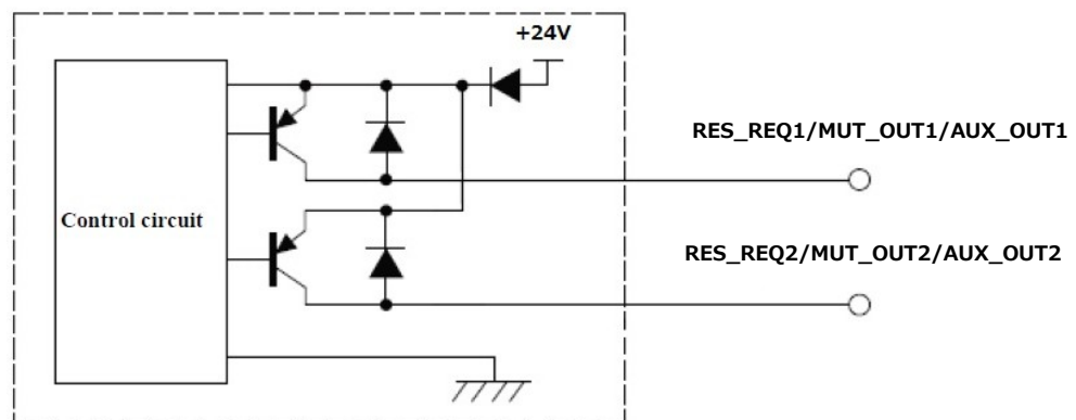
Figure 6-2 Output circuit
