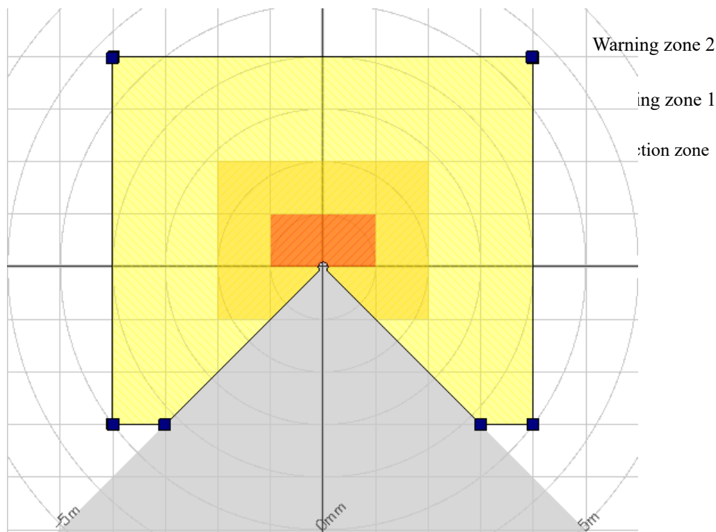
Figure 4-4 Warning zones
