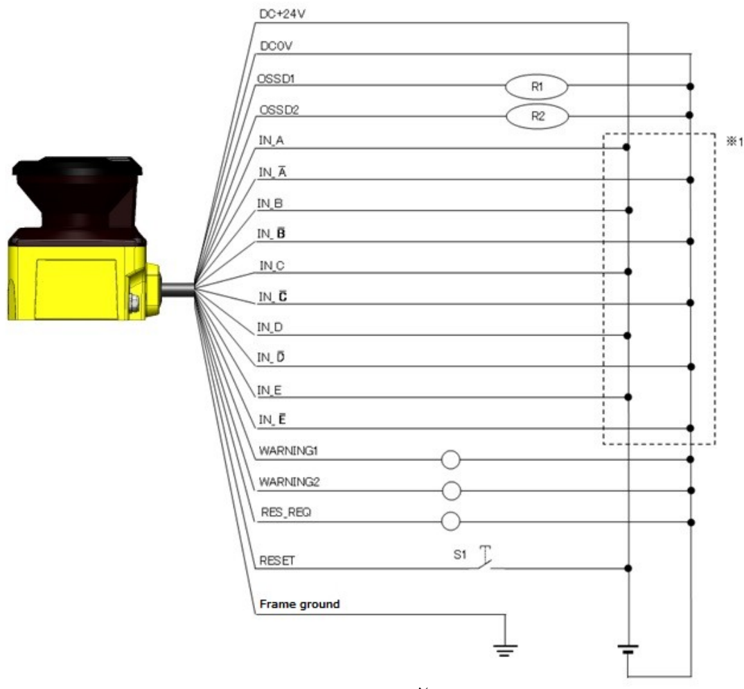
Figure 5-1 Wiring Example 1
